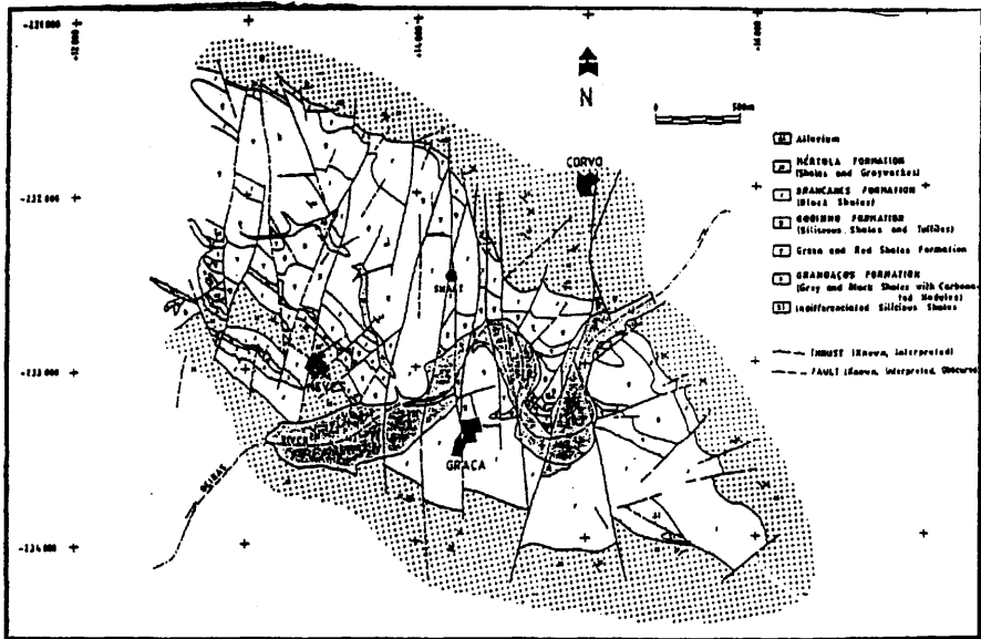
Figure 2. General geological map of Neves-Corvo mine area
